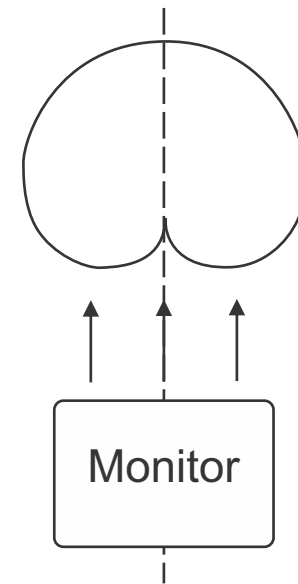
Cardioid Microphone Monitor Placement
