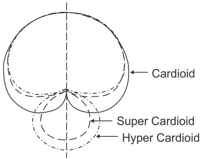
Microphone Patterns
